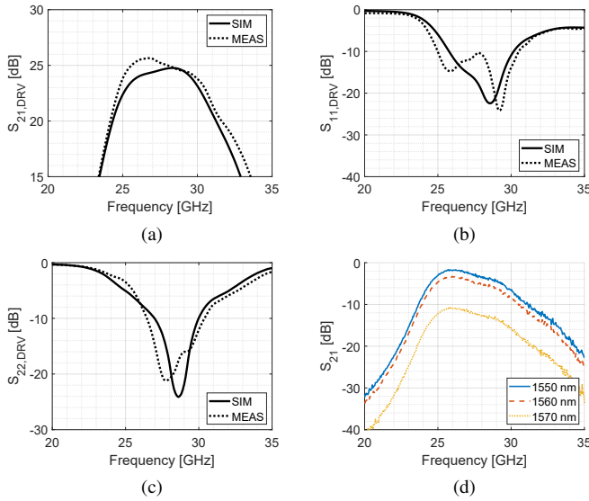
Fig. 12: (a)-(c) EAM driver S-parameters (d) Transfer function of the transmitter (2V driver supply, 1V EAM bias).
