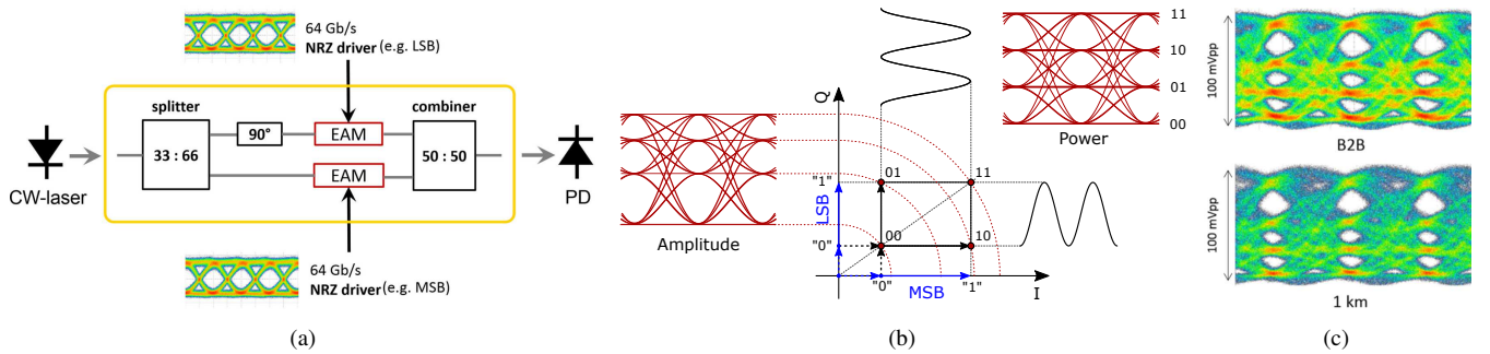
Fig. 1: 2-bit optical digital-to-analog converter (ODAC) for PAM-4 generation: (a) Operation principle; (b) Vector and eye diagrams; (c) Measured eye diagrams at 64 GBd in back-to-back (B2B) case and after 1km SSMF
