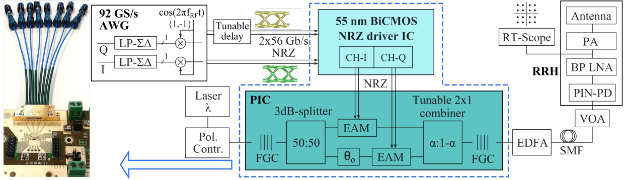
Fig. 17: Block diagram and experimental setup for the sigma-delta radio-over-fiber (SDoF) transmission using parallel EAMs.
