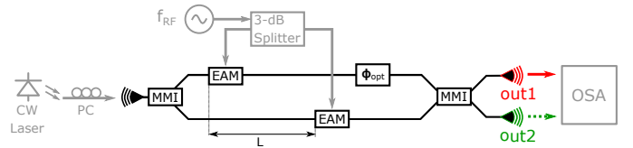
Fig. 20: OSSB generation with the quad-EAM structure (OSA: Optical spectrum analyzer).
