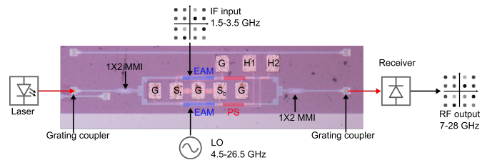
Fig. 25: Parallel EAM structure for upconversion.
