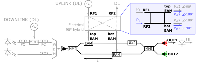
Fig. 24: Full duplex with the quad-EAM (MOD: Modulator, WDM: Wavelength division multiplexer; bot: Bottom).
