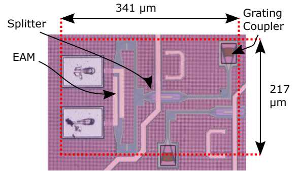
Fig. 8: Microscope image of the reflective EAM with modulator embedded in the loop mirror.
