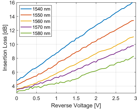
Fig. 9: Static insertion loss of the standalone 80\mu\text{m} EAMs.
