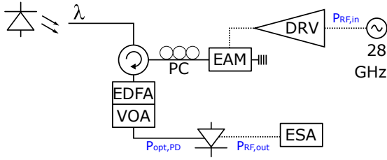
Fig. 15: Setup for 1dB compression measurement (ESA: electrical spectrum analyzer).
