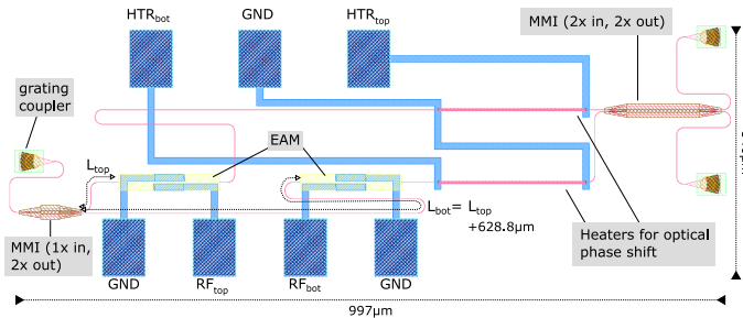
Fig. 19: Layout quadrature EAM for the 28 GHz band
