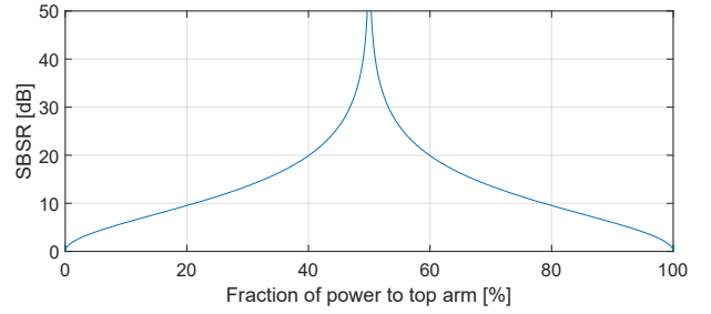
Fig. 23: Sideband suppression ratio (SBSR) as a function of power splitting ratio in the input MMI.
