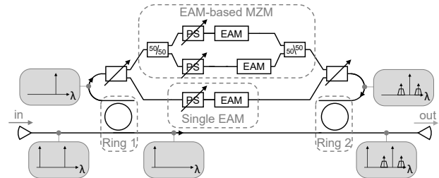
Fig. 26: Microring-assisted upconversion (PS: Phase shifter).
