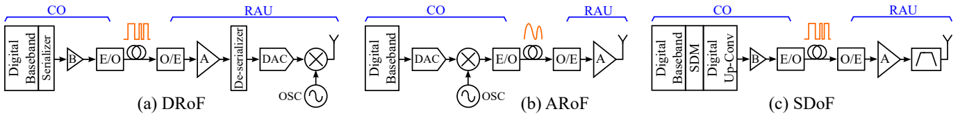
Fig. 16: RoF implementation types – B: Binary Driver; A: Amplifier; OSC: Oscillator; SDM: Sigma Delta Modulator.
