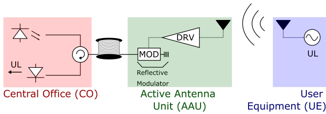
Fig. 6: Reflective implementation of the RFoF uplink path.
