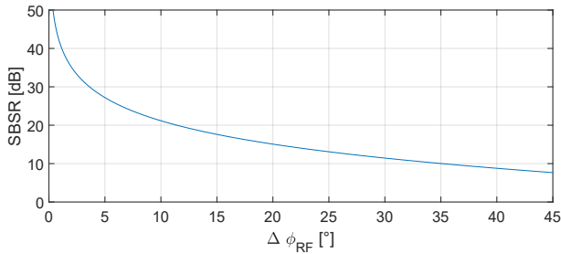
Fig. 22: Sideband suppression ratio (SBSR) as a function of deviation in the realized RF delay between the EAMs.
