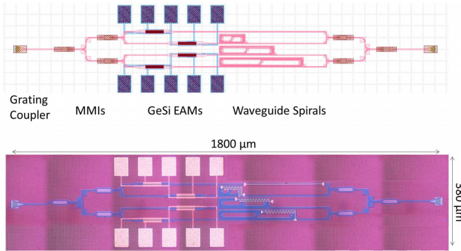
Fig. 3: Layout and microscope image of a 4:1 OTDM transmitter using EAMs
