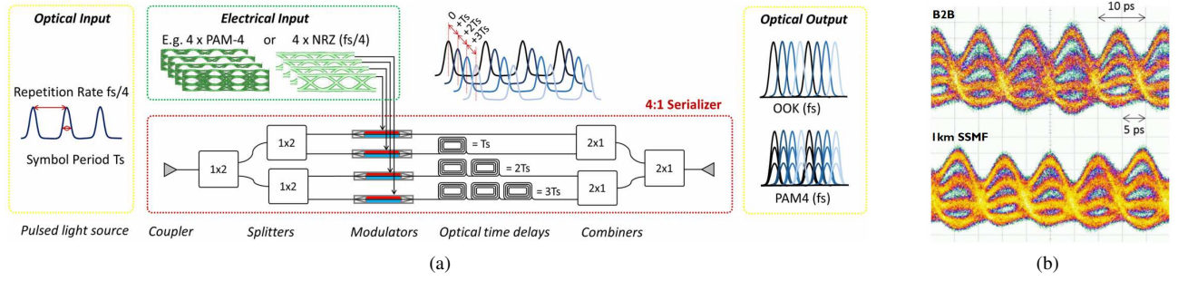
Fig. 2: Optical 4:1 serializer: (a) Operation principle; (b) Measured eye diagrams at 104 GBd in B2B and after 1km SSMF
