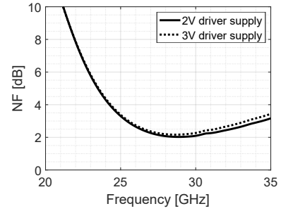
Fig. 14: Simulated noise figure of the RFoF transmitter.
