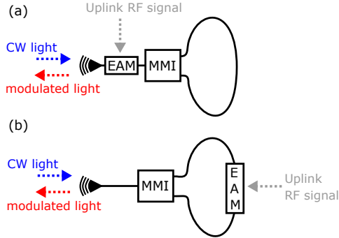
Fig. 7: Reflective EAM: (a) EAM in front of the loop mirror; (b) EAM embedded in the loop mirror.
