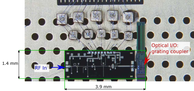
Fig. 11: Reflective 28 GHz RFoF transmitter.
