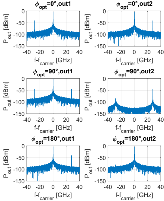
Fig. 21: Simulated output spectrum given \phi_{opt} relative optical phase difference and equal RF input at both EAMs.
