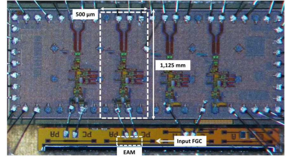
Fig. 5: Silicon integrated EAM PAM-4 receiver.
