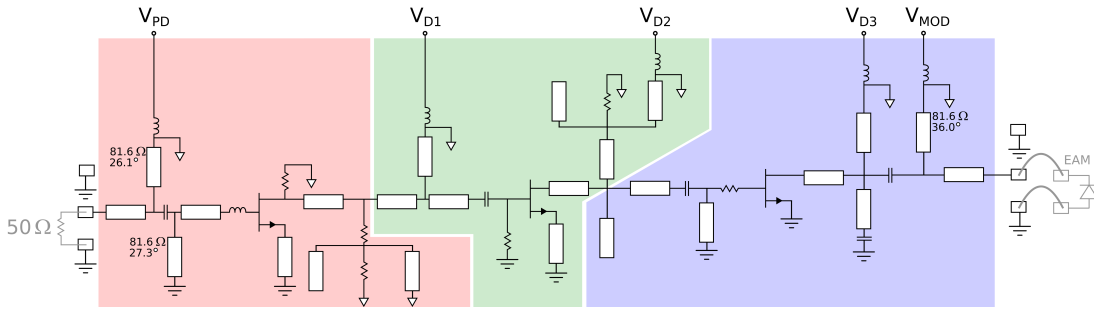
Fig. 10: Overall schematic of the 3-stage narrowband EAM driver.
