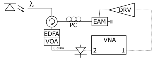
Fig. 13: Setup for S_{21} characterization (PC: polarization controller; DRV: driver; VOA: variable optical attenuator).
