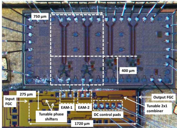
Fig. 4: Silicon integrated EAM PAM-4 transmitter.
