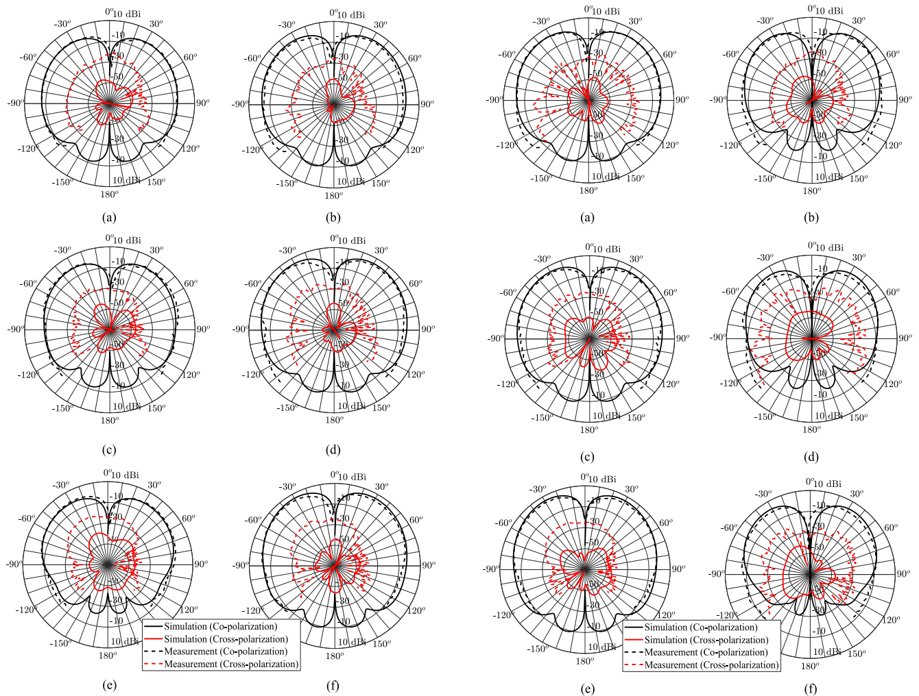
Figure 18. Radiation patterns at 5.15 GHz in (a) the XZ-plane and (b) the YZ-plane, at 5.50 GHz in (c) the XZ-plane and (d) the YZ-plane, at 5.85 GHz in (e) the XZ-plane and (f) the YZ-plane for the bias current set to +10 mA, meaning that the antenna exhibits y -oriented linear polarization.
