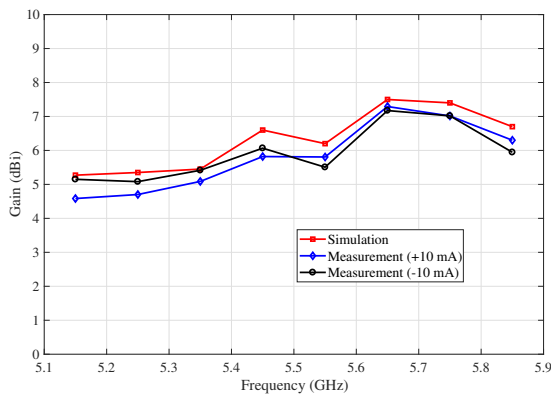
Figure 17. Measured and simulated maximum gain across the operating band in two polarization states: y -oriented linear polarization (bias current of +10 mA) and x -oriented linear polarization (bias current of -10 mA).
