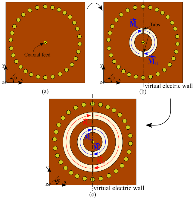
Figure 2. Design evolution of a single-feed AFSIW cavity-backed slot antenna with ultra-wide bandwidth and conical-beam radiation pattern. (a) Step 1: Circular cavity fed by a coaxial probe at its center. (b) Step 2: Linearly-polarized radiation is obtained by inserting a resonant annular ring slot in the top plane of the cavity and exploiting two diametrically positioned shorting tabs. (c) Step 3: Additional radiating ring with shorting tabs is positioned to improve impedance bandwidth of the antenna.
