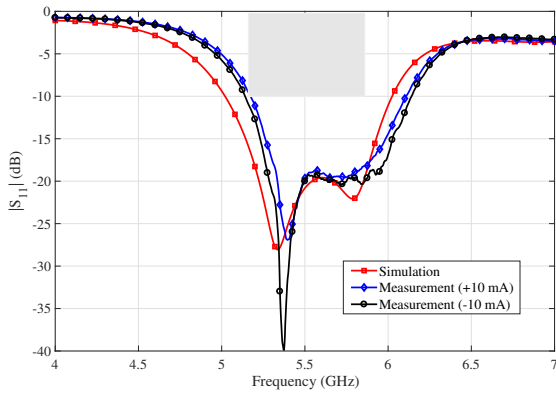
Figure 15. Magnitude of input reflection coefficient |S_{11}| in two operating states: y -oriented linear polarization (bias current of +10 mA) and x -oriented linear polarization (bias currents of -10 mA).
