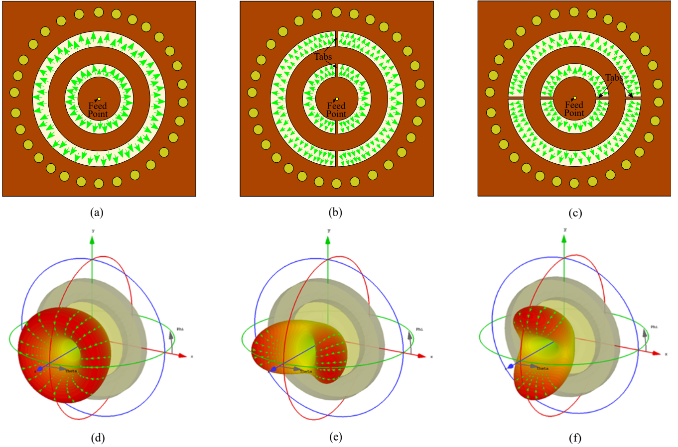
Figure 5. AFSIW cavity-backed slot antenna: (a) without symmetrically positioned shorting tabs, (b) with shorting tabs oriented in yz - plane ( x -oriented polarization state), (c) with shorting tabs oriented in xz - plane ( y -oriented polarization state). 3D gain pattern of the antenna on a linear scale. In all gain patterns, the |E_\theta| is the main component of the electric field ( |E_\varphi| \ll |E_\theta| ). (d) A circular AFSIW cavity-backed annular slot antenna without shorting tabs. Proposed circular AFSIW cavity-backed annular slot antenna with shorting tabs: (e) x -oriented polarization state, (f) y -oriented polarization state.
